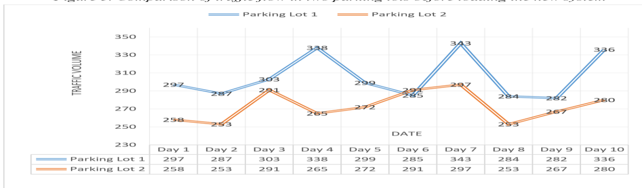
Figure 6. Comparison of traffic flow between two parking lots after loading the new system in parking lot 1 From Figure 5, it can be seen that the traffic flow of the two parking lots before loading the new system is actually similar. Within the ten days selected for the experiment, the average traffic flow of parking lot 1
