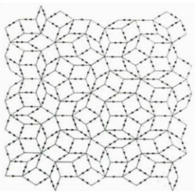
Figure 2: P3 Penrose tiling formed with thick and thin rhombuses, following the matching rule.
