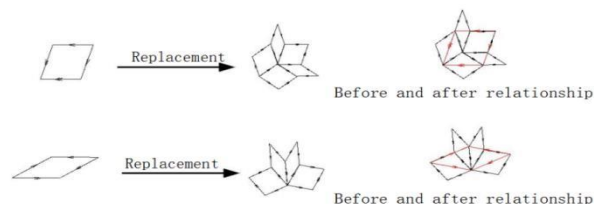
Figure 3: Construction rules for P3 Penrose tiling (starting with a thick rhombus and a thin rhombus, respectively).
