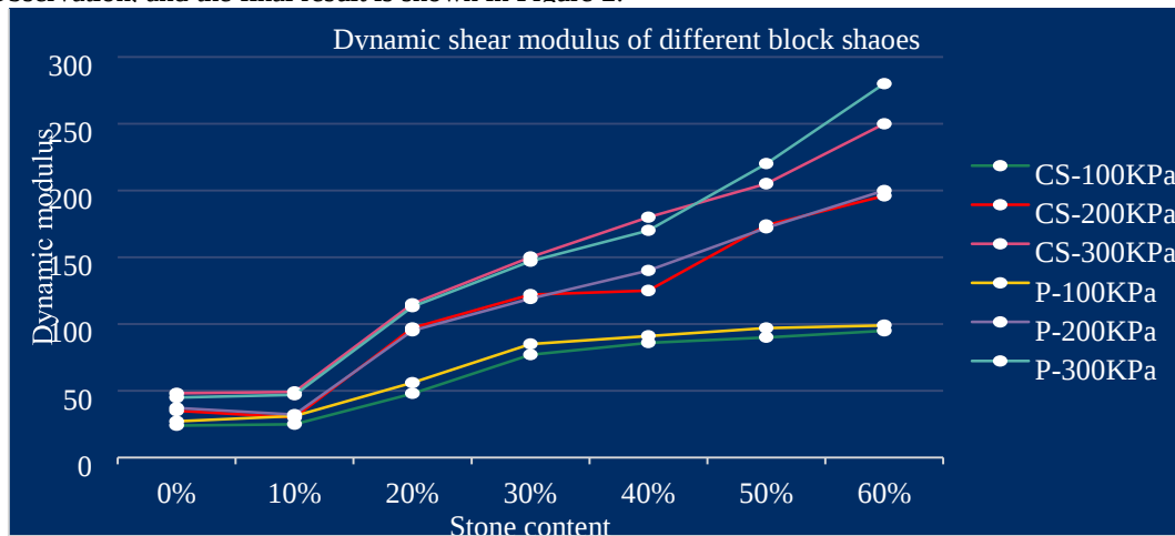
Figure 2. Dynamic shear modulus changes of different rock shapes
