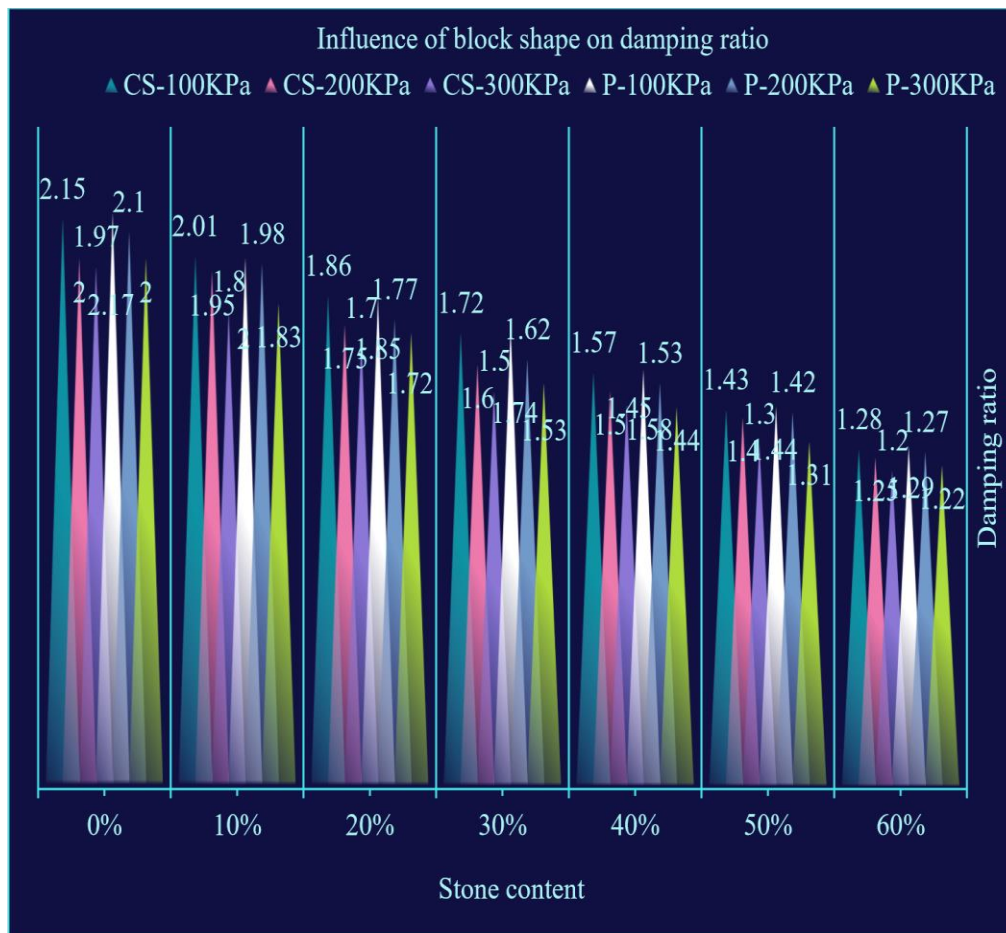
Figure 3. The influence of block shape on damping ratio
