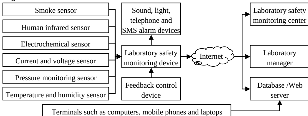
Figure 4: Architecture of laboratory safety monitoring and control system
