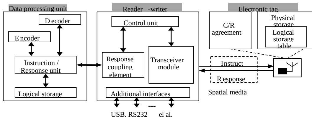
Figure 2: RFID system composition
