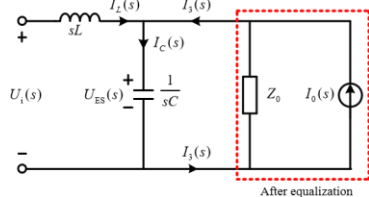
(b) Equivalent S-domain model
