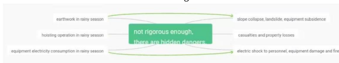
Figure 3 Mind map
