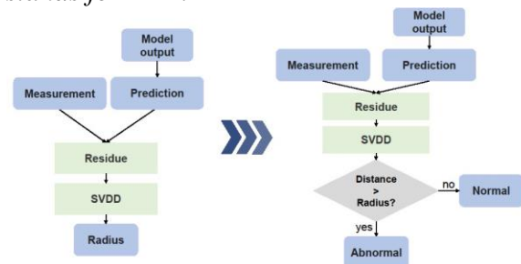
Figure 3: DKNN based anomaly detection protocol.
