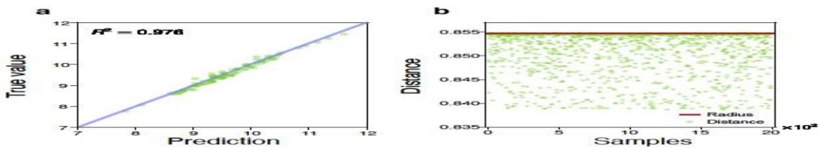
Figure 5: DKNN process monitoring for Example 1 based on mean-value data. (a) shows the DKNN model based on mean-value data cast precise one-step predictions, as predictions (green dots) are
