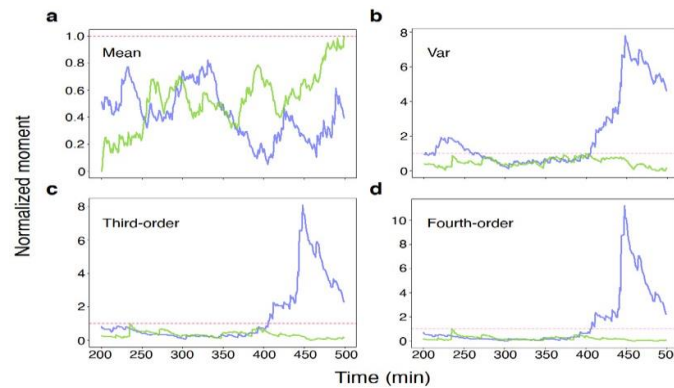
Figure 6: Sensitivity of moments against anomaly. The anomaly occurs at time t = 401 . All the moments are normalized for visual convenience, and the normalization methods are stated in Appendix 6.2. Moments of order higher or equal to 2 are sensitive to anomaly, while the mean value is not.
