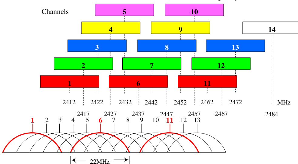
Figure 1: Channel planning of 2.4GHz spectrum
