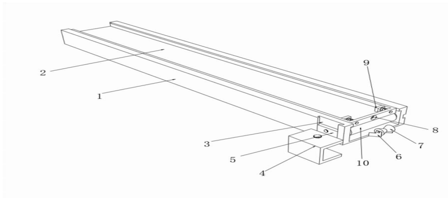
Figure 1: Schematic Diagram of the Experimental Apparatus
