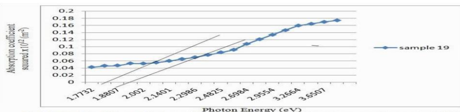
Fig. 7b: Graph of absorption coefficient squared versus photon energy for sample 19 (65°C)
