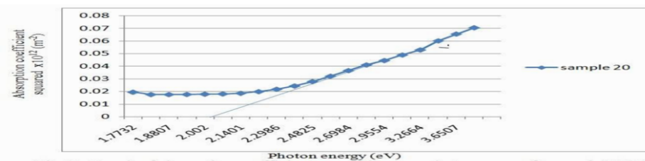
Fig. 7c: Graph of absorption coefficient squared versus photon energy for sample 20 (70°C)
