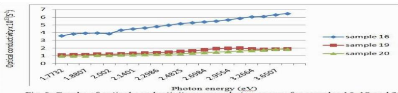
Fig. 5: Graphs of optical conductivity versus photon energy for samples 16, 19 and 20
