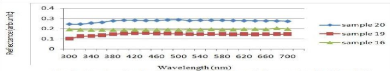
Fig. 4: Graphs of reflectance versus wavelength for samples 16, 19 and 20
