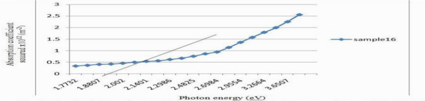
Fig. 7a: Graph of absorption coefficient squared versus photon energy for sample 16 (50°C)
