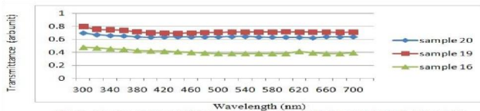
Fig. 3: Graphs of transmittance versus wavelength for samples 16, 19 and 20
