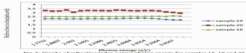
Fig. 6: Graphs of refractive index versus photon energy for samples 16, 19 and 20
