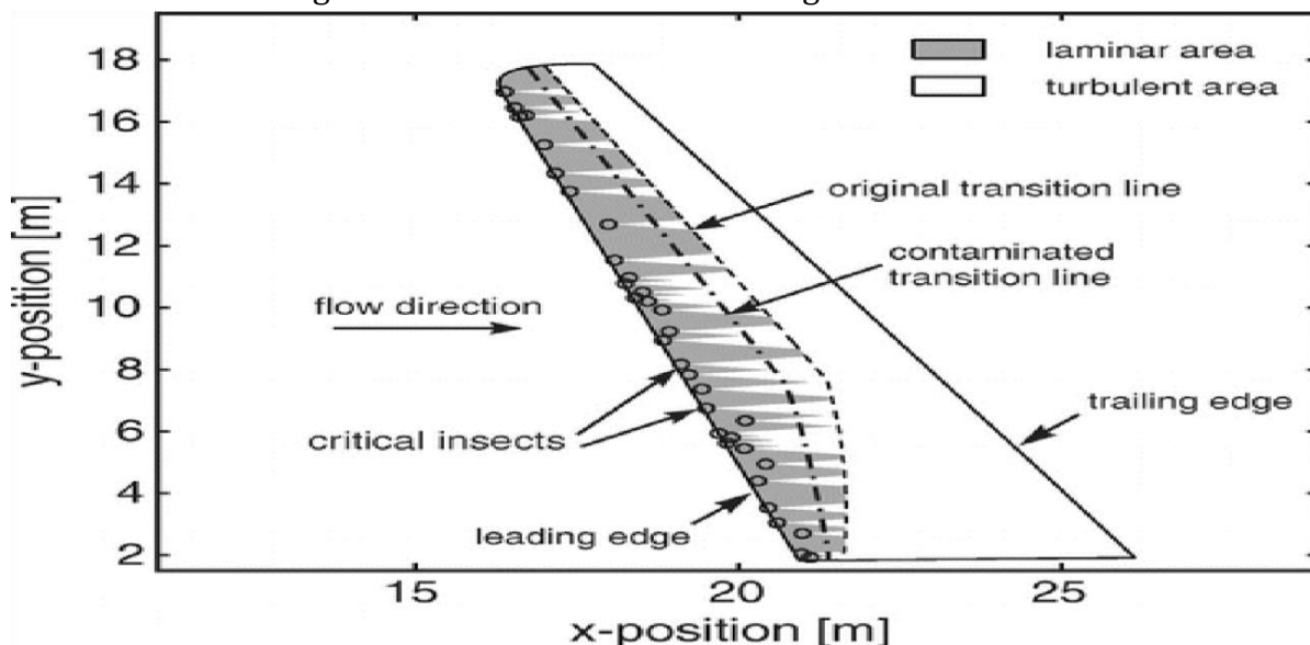
Figure 5: Impact of insect contamination on laminar flow
