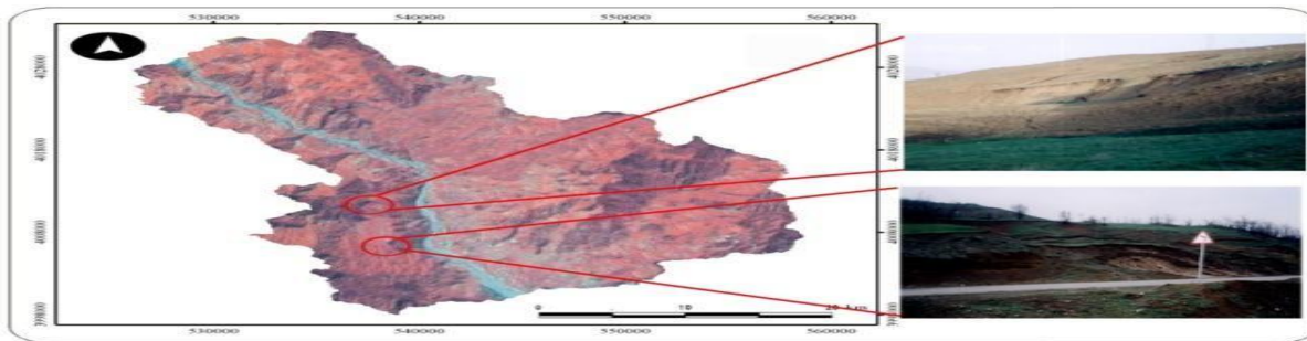
Fig.4. SPOT satellite images at the central Zab basin landslide
