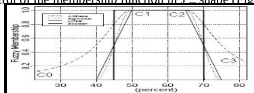
Fig.3. J-Shape function in fuzzy set
