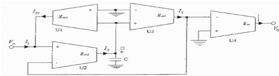
Fig-6 First order active low pass filter using multiple OTA (second method)
