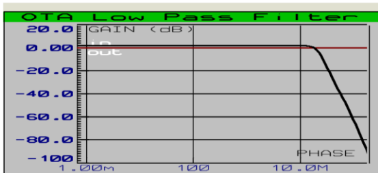
Fig. 8 Frequency response of Proteus professional 7 simulated OTA Low pass filter circuit, with pass band up to 121MHz at -10dB of gain. Maximum gain is 2dB for bias current of g_{m1} = 10\text{mA} and g_{m2} = 5\text{mA} for case -3: The bias current of g_{m1} is less than bias current of g_{m2} results are absurd.
