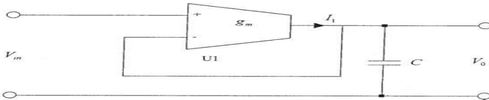
Fig-5 First order active low pass filter using single OTA (First method)
