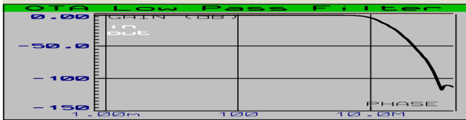
Fig. 8 Frequency response of Proteus professional 7 simulated OTA Low pass filter circuit, with pass band up to 18MHz at -10dB of gain. Maximum gain is 2.59dB, For bias current of 5mA ( i.e g_{m1} = g_{m2} = 5\text{mA} )
