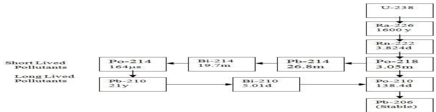
Fig.: Uranium Decay Series showing radon (the only gaseous member of the series) and its daughter products.
