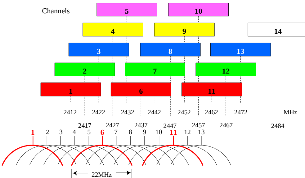
Figure 1: Channel planning of 2.4GHz spectrum
