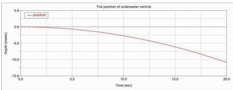
Figure 4: The relationship between the position of AUV's center of mass and time when AUV ascent. Figure 4 shows that when the direction of depth increase is taken as the positive direction, it can be known that the AUV accelerates upward under the action of the set oscillating velocity of the steering gear.
