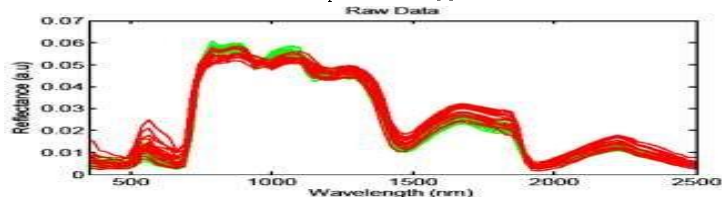
Figure 1. Spectral reflectance of the representative field data from 350-2,500 nm.
