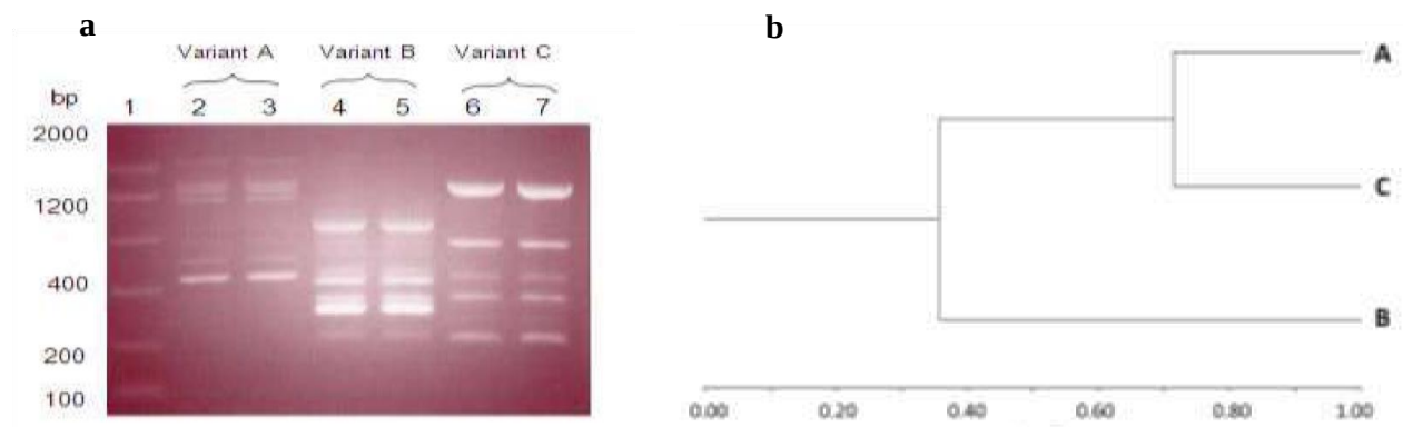
Figure 2. PCR-RAPD products of three variants of S. lemuru (a). Number 1 is DN A standard; number 2 and 3 are variant A; 4 and 5 are variant B; 6 and 7 are variant C of S. lemuru on 2% gel Agarosa. The phylogenetic tree of S. Lemuru in Lombok Strait (B).
