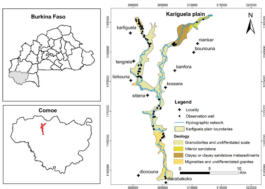
Figure 1: Location of the Karfiguélé plain in Burkina Faso, showing the extent, geology and locations of the river, observation wells, villages.
