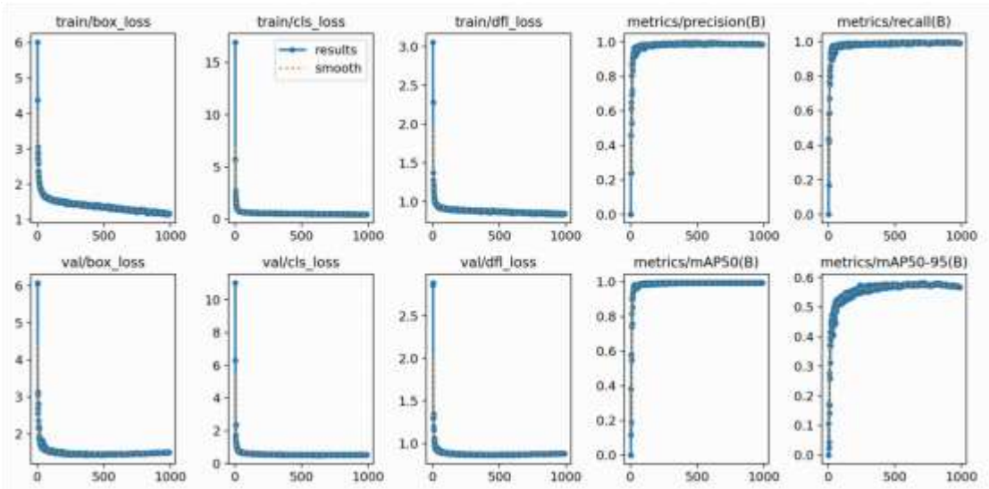
Figure 3-2 Training data of taillight recognition model
