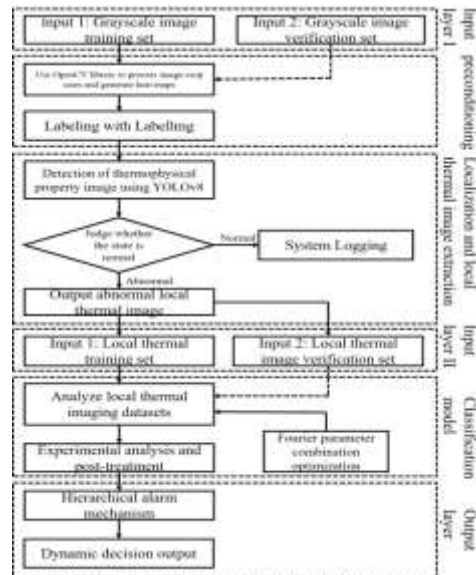
Figure 2-2 Thermal physical property image recognition technology architecture
