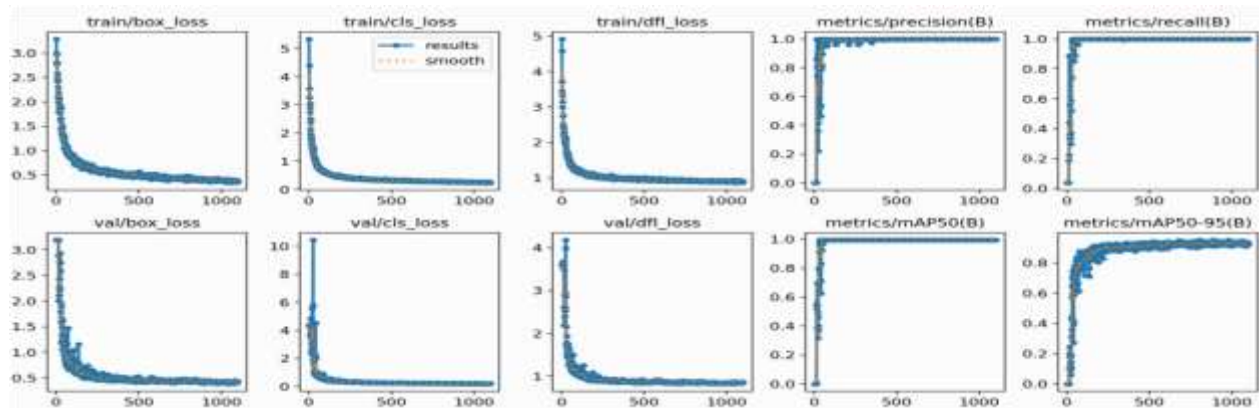
Figure 4-3 Training data of animal recognition model
