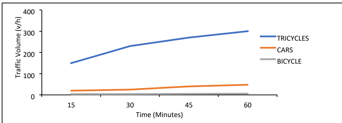
Fig.1: Hourly Traffic Variations, Morning Peak Period (8:00 – 9:00am)
