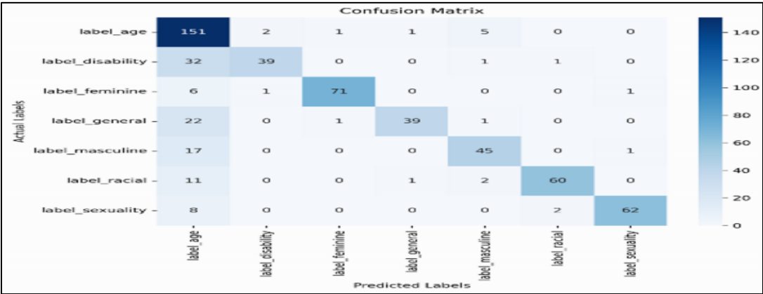
Figure 3: RoBERTa Confusion Matrix
