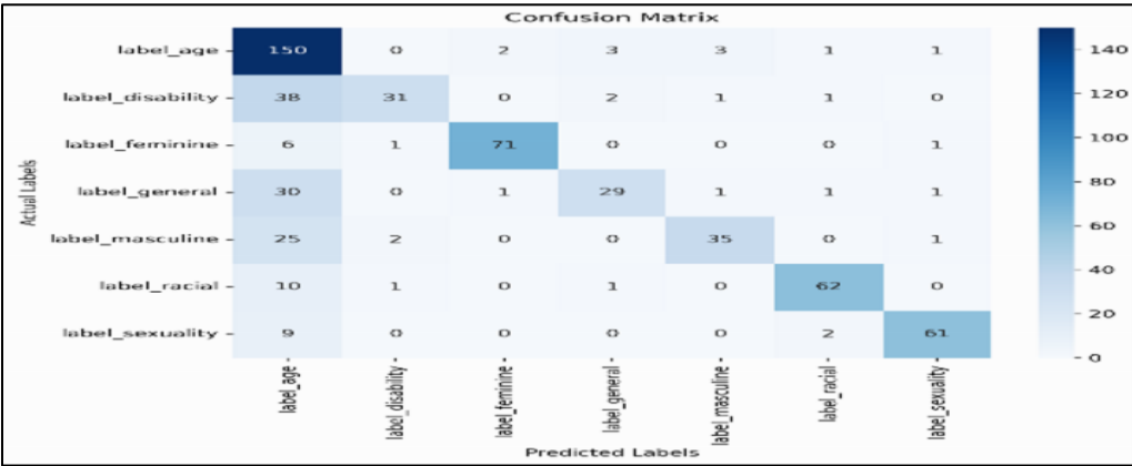
Figure 2: BERT Confusion Matrix
