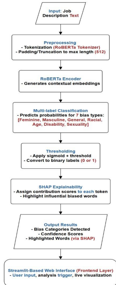
Figure 1: Flowchart of the Bias Detection Process.
