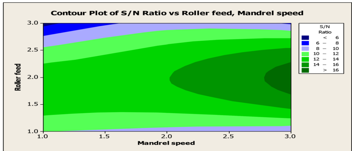
Figure 4: Contour plot of roller feed and mandrel speed on Ovality
