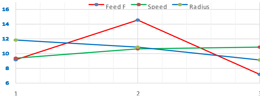
Figure 2: Main effects of process parameters on Ovality
