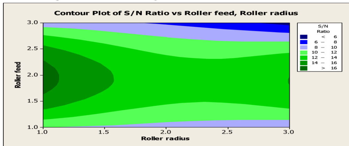
Figure 5: Contour plot of roller feed and roller radius on Ovality
