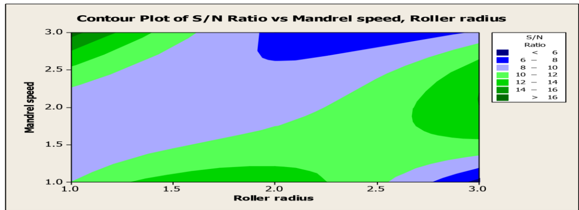
Figure 6: Contour plot of mandrel speed and roller radius on Ovality
