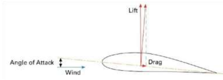
Figure 1: Lift & drag vectors, from WE handbook (no date) [3]
