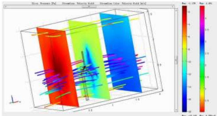
Figure 16 Pressure and streamline in 5 m/s maximum inlet speed in Case 2
