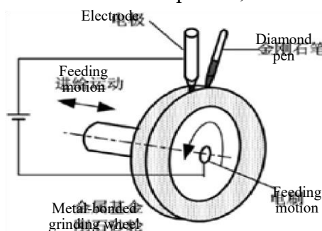
Fig.1 wire electrical discharge machining technique [7]
