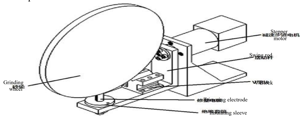
Figure. 2 Structure of the electric spark dressing device
