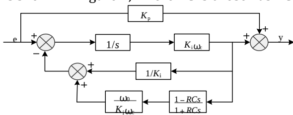
Figure 4: QPCI control block diagram using all-pass filter.
