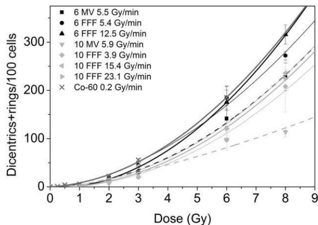
Figure 3. Calibration curves for dicentric + rings caused by LINAC X-ray irradiation, regarding dose and response. Lines depict the predicted curves of the linear quadratic model.
