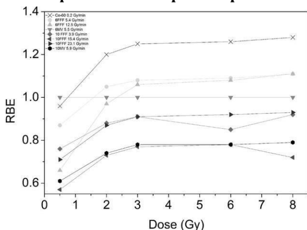
Figure 4. The following examples show average RBE values for different photon energies as a function of dose: 60 Co \gamma 0.2 Gy/min, 6 FFF (5.4-12.5 Gy/min), 10 MV (5.9 Gy/min), and 10 FFF (3.9-23.1 Gy/min).
