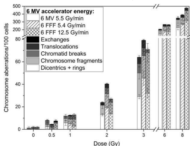
Figure 1. Human blood cells from two donors were exposed to a 6 MV/FFF photon beam at several dosage rates; it shows the frequencies of dicentric + rings, chromosomal fragments, translocations, and overall aberrations.
