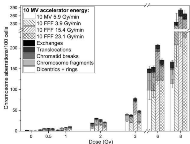
Figure 2. Dicentric + rings, chromosomal fragments, translocations, and overall aberration frequencies in human blood cells from two donors exposed to varying dosage rates of a 10 MV/FFF photon beam.
