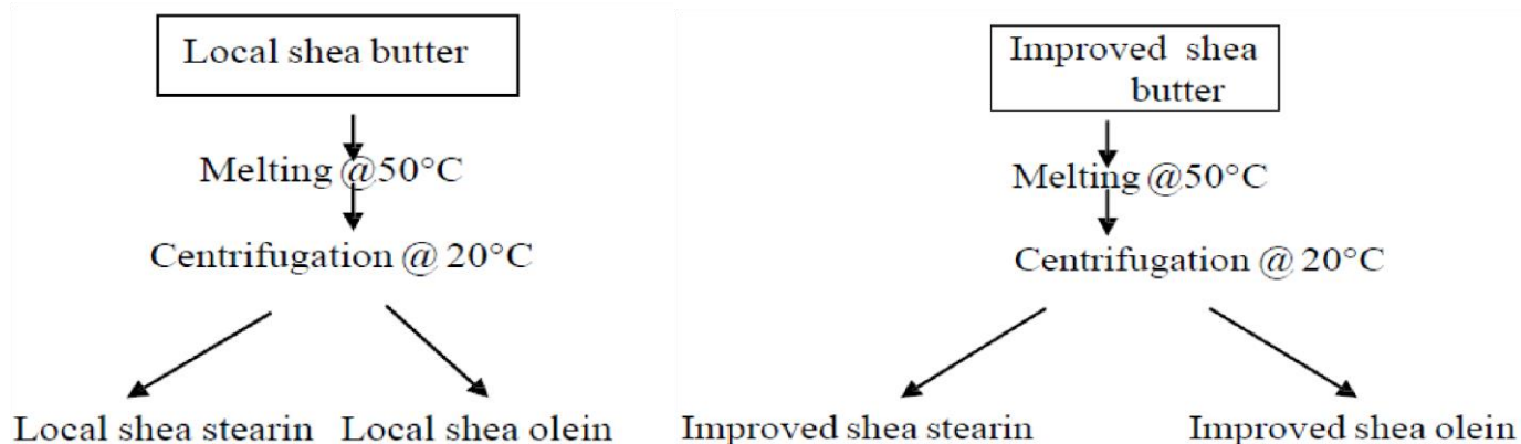
Figure 2. Flow chart for fractionation of shea butter into olein and stearin. Source: Addaquay (2004).
