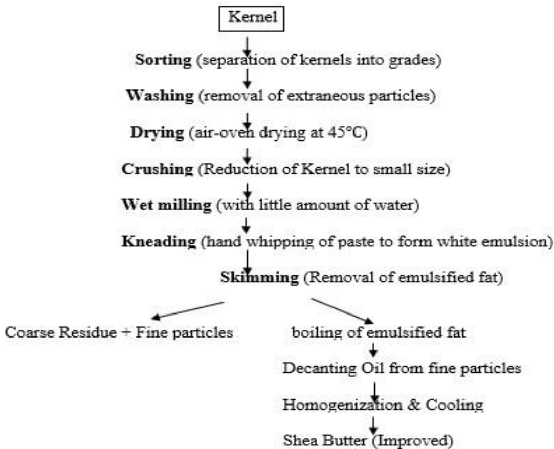
Figure 1. Improved method of Extraction of shea butter (Source: ARSO, 2011).
