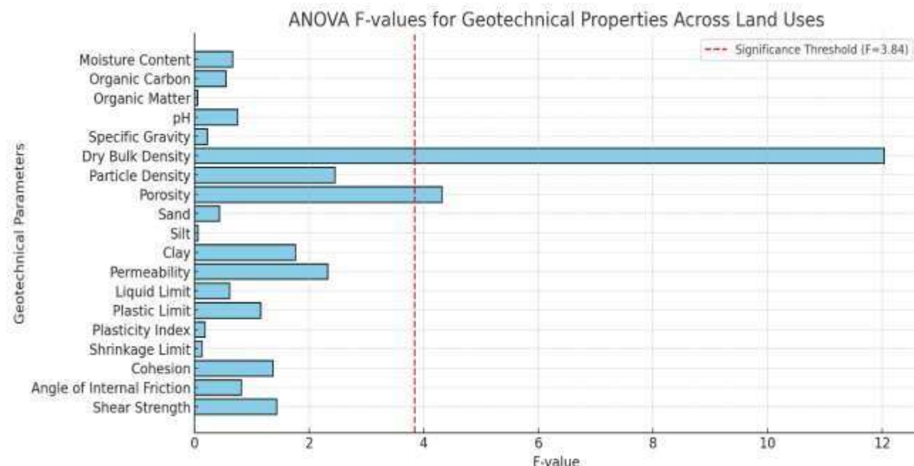
Figure 1: ANOVA F – Values Comparison of Geotechnical Properties across Land Uses Bar Chart of ANOVA F-values for the 19 geotechnical parameters under investigation. The red dashed line represents the significance threshold ( F = 3.84 at \alpha = 0.05 ). Parameters exceeding this threshold, such as Dry Bulk Density (12.03) and Porosity (4.32), indicate statistically significant differences among land uses.
