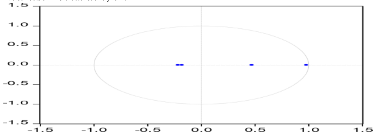
Figure 4.5: Dynamic Stability.
