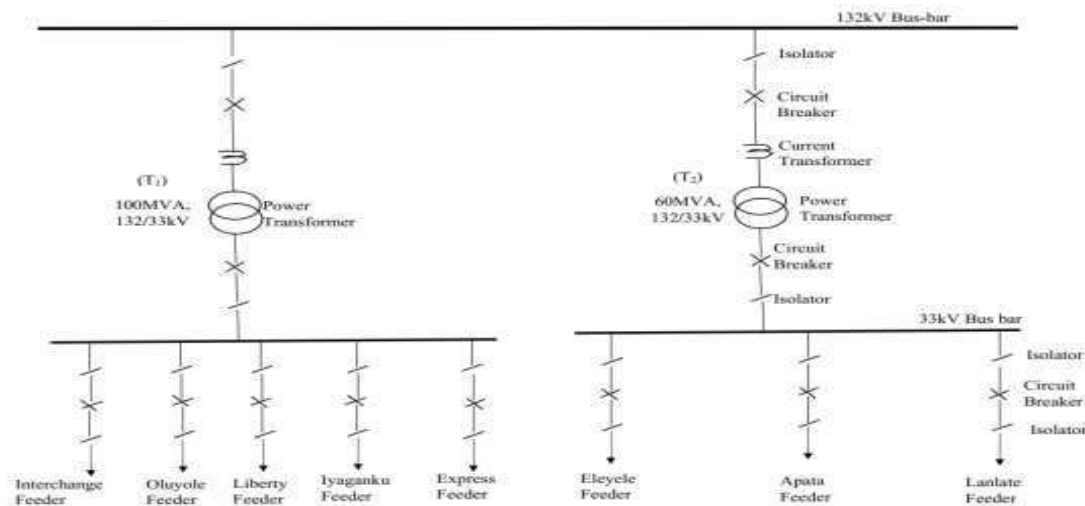
Figure 1: Schematic Diagram of 132/33kV Ayede Transmission Sub-Station
