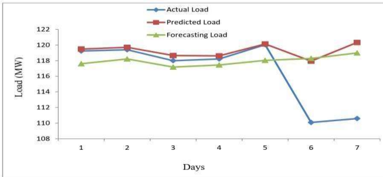
Figure 6: Total Forecasting Load between 1 to 7 , May 2023 (raining season)
