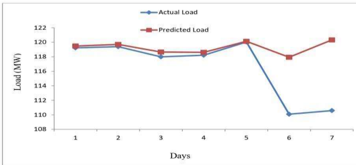
Figure 5: Total Predicted Load between 24 to 30 April, 2023 (raining season)
