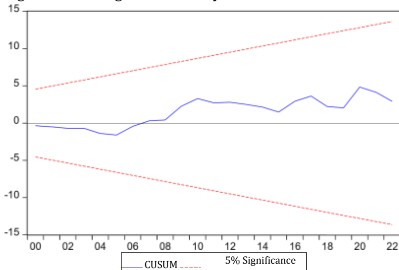
Figure 3.8: CUSUM Stability Test for ARDL (1,2,0,3,4)
