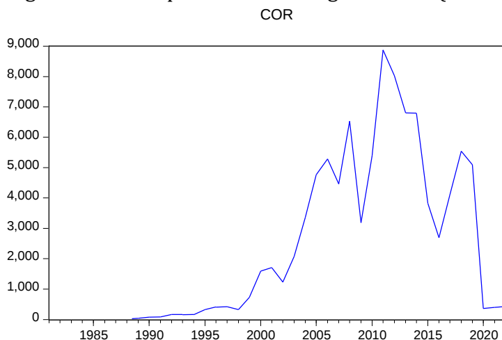
Figure 3.3: Time plot of Annual Nigerian COR (1981 – 2022)
