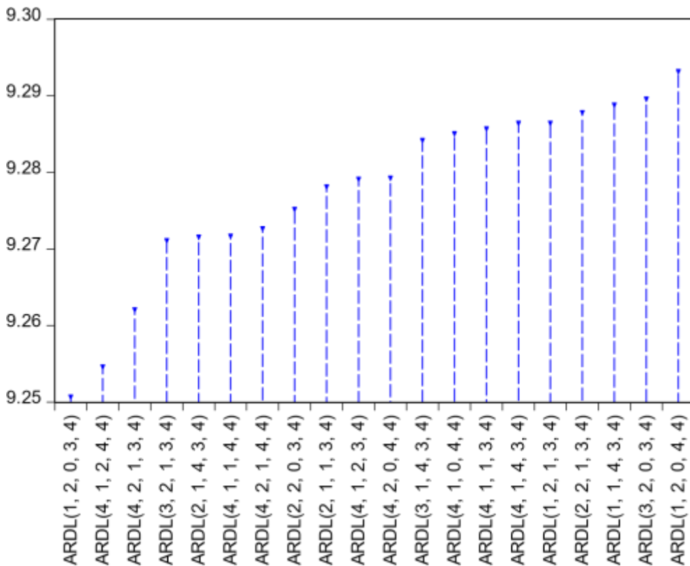
Figure 3.6: ARDL Model Selection (Using GDP as Dependent Variable)
