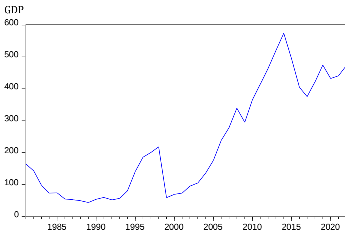
Figure 3.1: Time plot of Annual Nigerian GDP (1981 – 2022)
