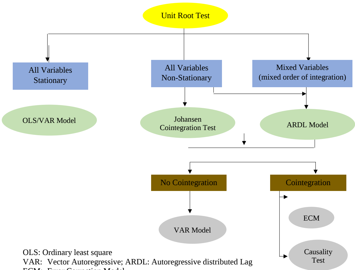
Figure 1: Methodology Selection Flow Chart for Time Series Data
