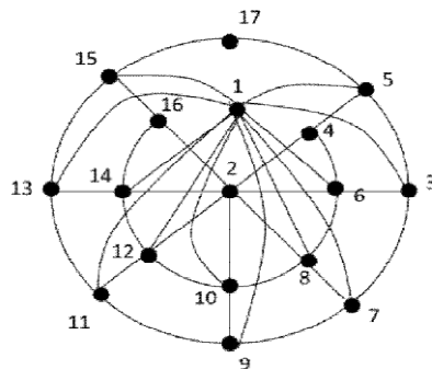
Figure: 6 Switching of vertex w in C_{19}
