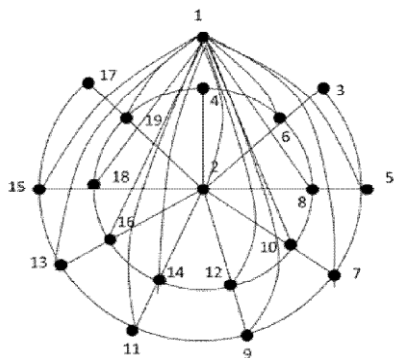
Figure: 5 Switching of w in C_{19}
