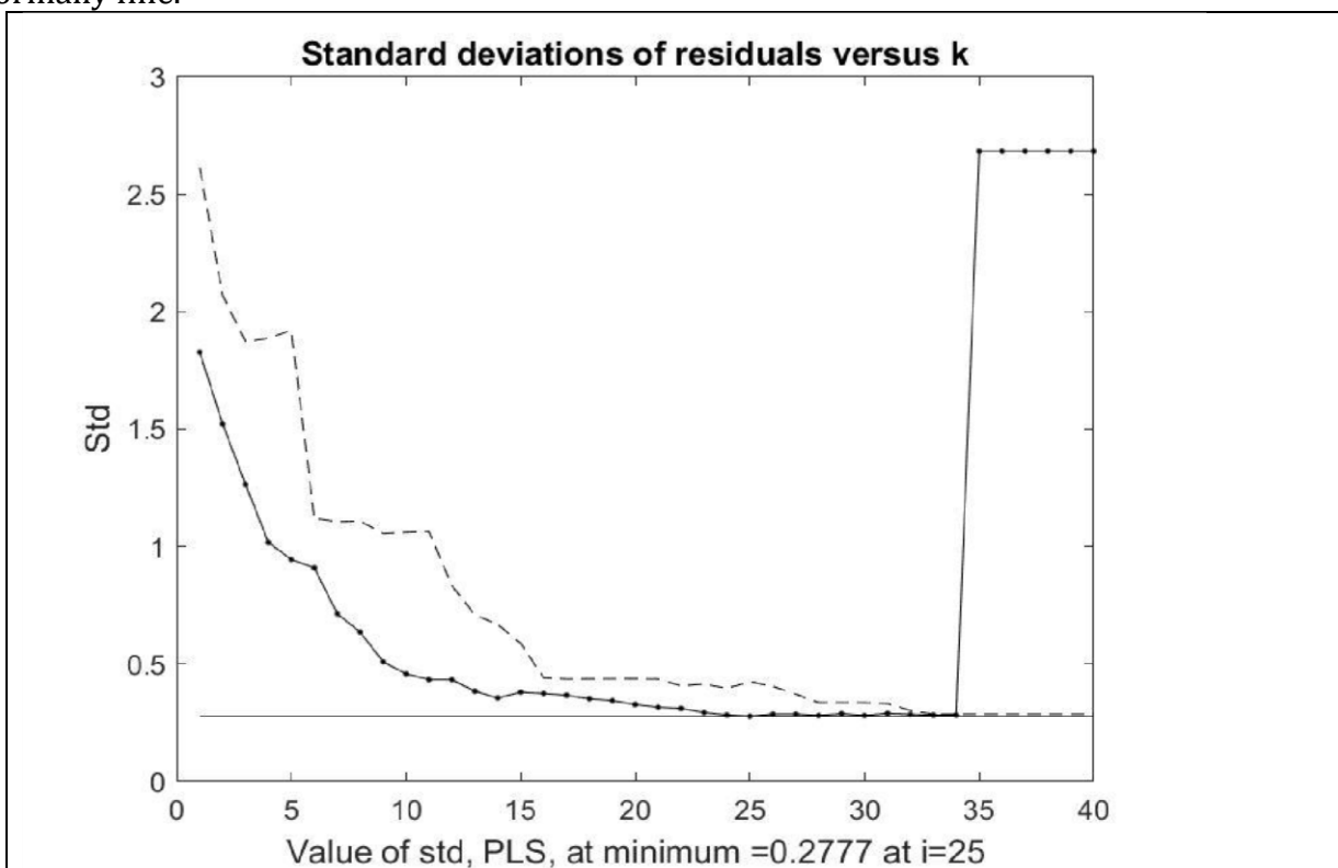
Figure 3. Plot of the standard deviations of residuals, s_t for PLS .-, and s_r for RR --. x-axis is the dimension. Spectral data.
