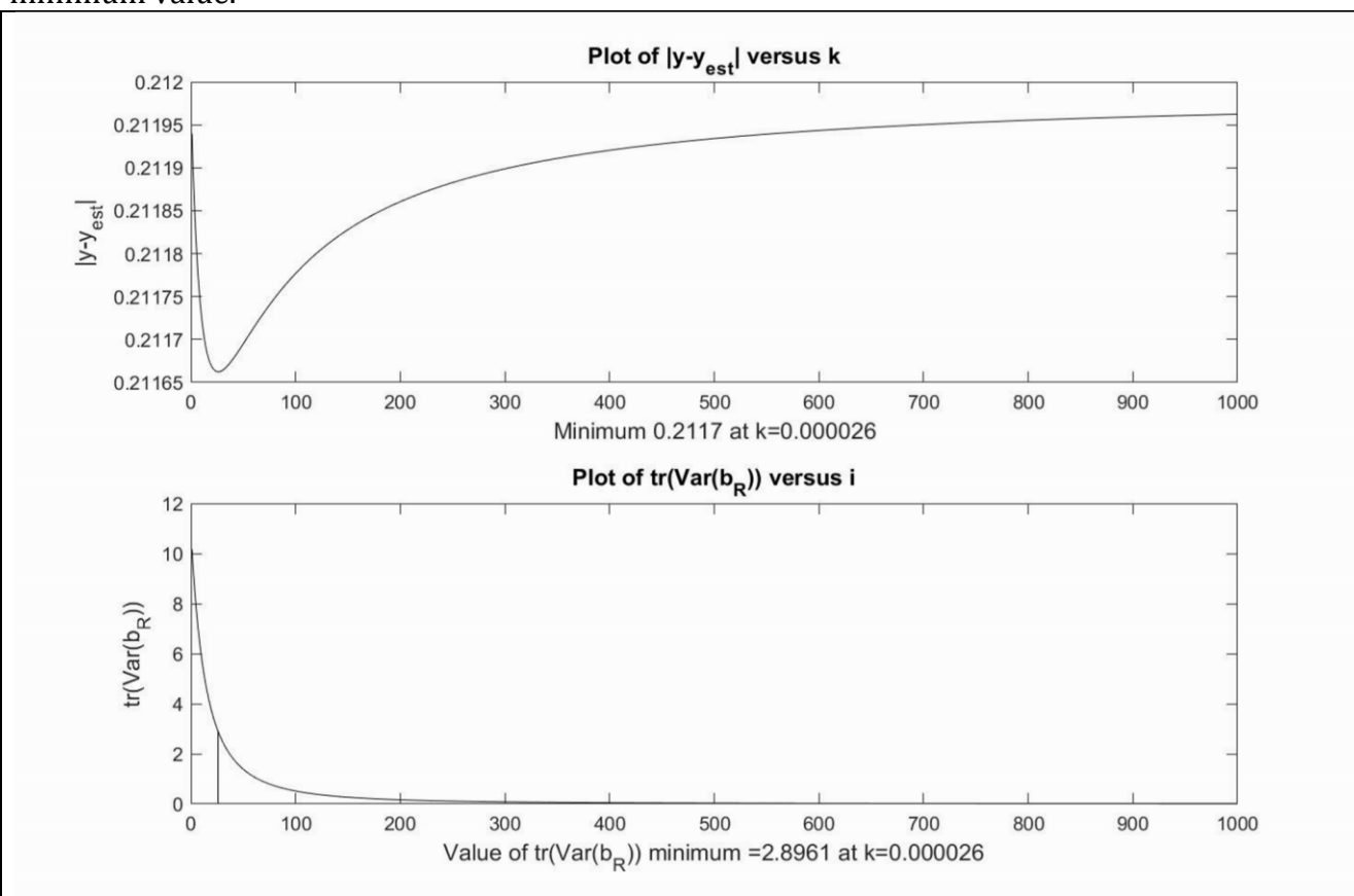
Figure 1. Upper figure plot of |\mathbf{y} - \hat{y}_{est}| versus k . k = i \times 10^{-6} , i = 1, 2, \dots, 10^4 . x-axis is the i -values. The lower figure is plot of \text{tr}(\text{Var}(\mathbf{b}_R)) , (8), versus k . Process data.
