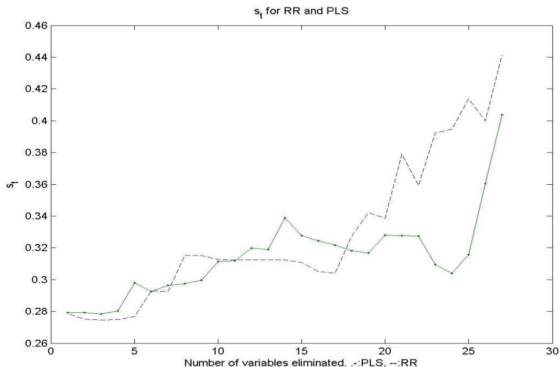
Figure 4. The values of s_t were obtained for RR and PLS at the backwards deletion of variables. .- is those from PLS, -- from RR.
