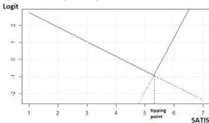
Figure 2. A Graphic Representation of the Piecewise Logistic Regression Result
