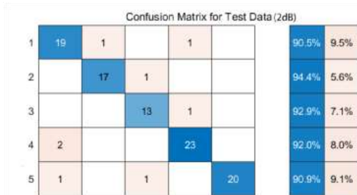
Figure 4: Confusion matrix for test data (2dB)
