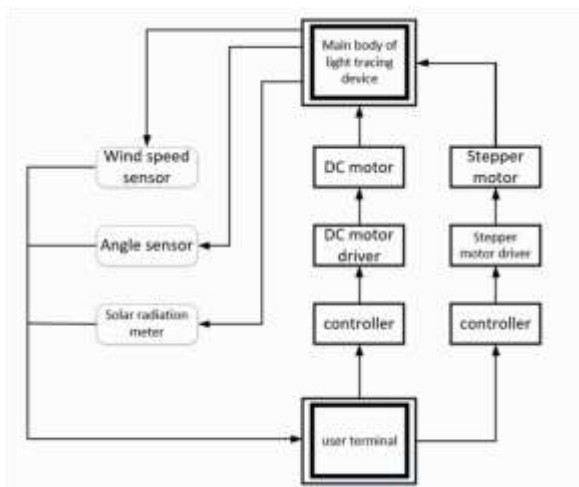
Figure 1: System Structure
