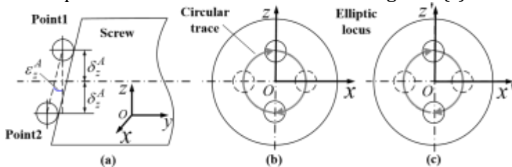
Figure 4: Schematic for assembly error of screw shaft.
