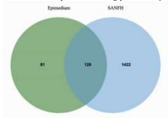
Figure 1: Venn diagram.
