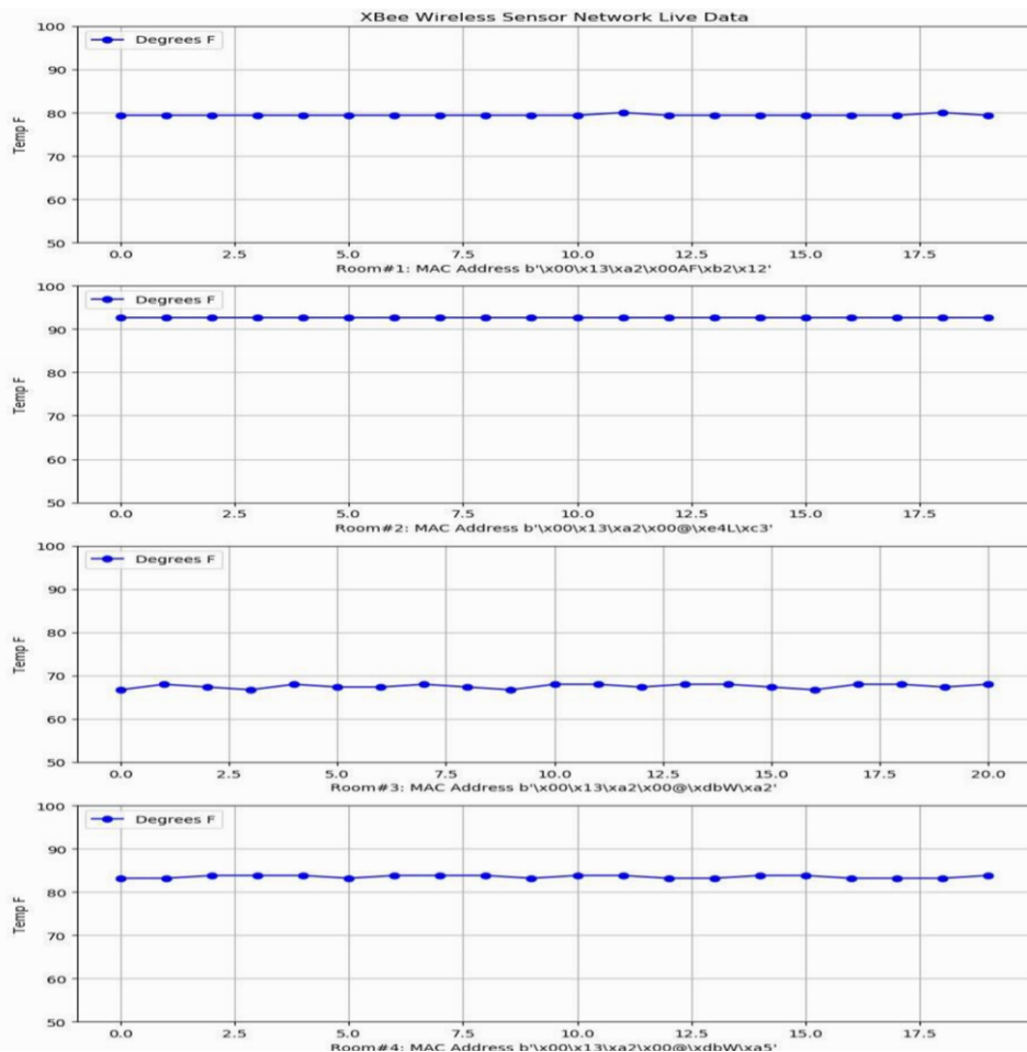
Figure 7. Live data visualization in sequential order using Matplotlib.
