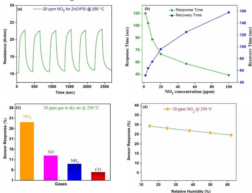
Figure 6: (a) The cyclability test up to 6th cycles at 20 ppm \text{NO}_2 level in dry air, (b) Shows the variation in response and recovery times with different concentrations (2 ppm–100 ppm) of \text{NO}_2 at 250^\circ\text{C} for ZnO/PSi sensor, (c) Cross sensitivity test at 20 ppm concentration of various gases and (d) Depicts the response versus humidity curve at 20 ppm of \text{NO}_2 for proposed ZnO/PSi sensor.
