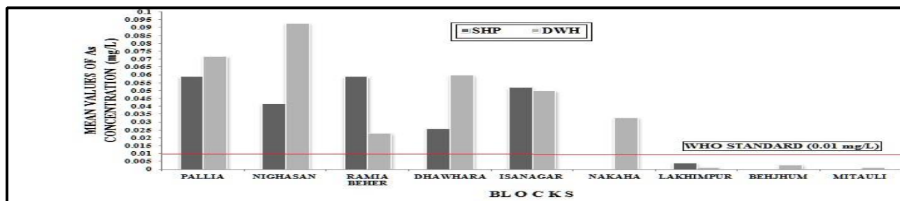
Figure 1: Comparison of mean values of Arsenic (T) concentration from Uttar Pradesh.
