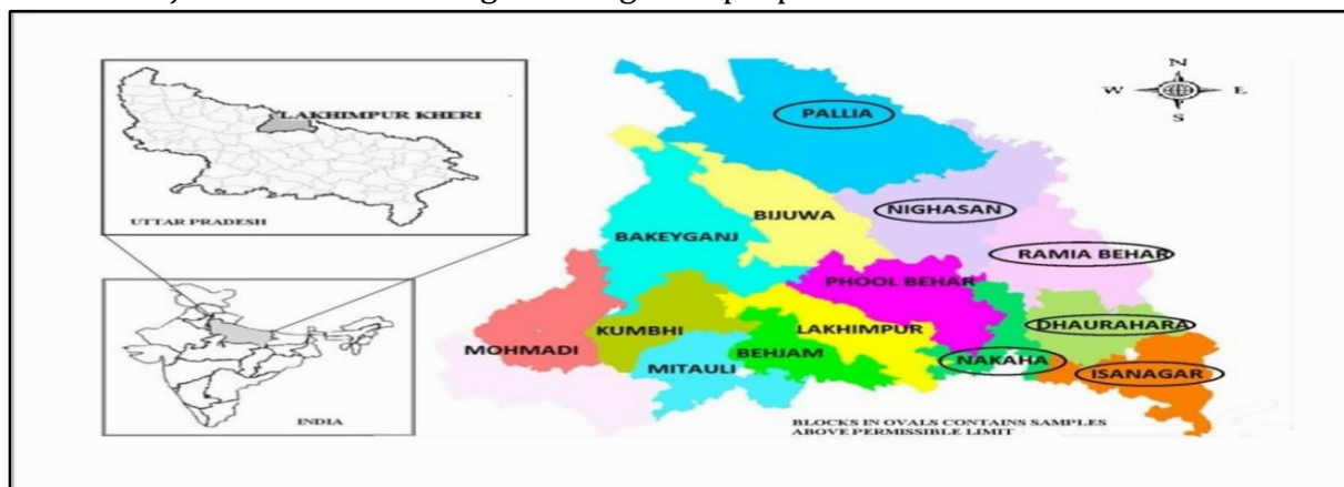
Figure 1: Location map of study area showing all 15 sampling blocks of Lakhimpur Kheri district, Uttar Pradesh, India. (Highly contaminated areas shown in oval)
