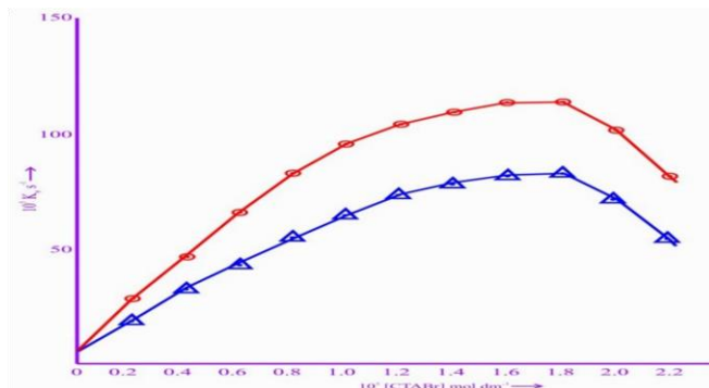
Fig. 2. Reaction of bis-4-CDMPP with \text{H}_2\text{O}_2 in presence of CTABr.
