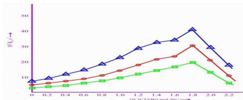
Fig. 1. Reaction of 4-CDMPP with \text{OH}^- ions in presence and absence of CTABr at 40 \pm 0.5^\circ\text{C} .
