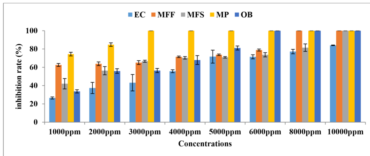
Figure 1: Activity of essential oils on the mycelial growth of Colletotrichum gloeosporioides (n = 120, P = 2e-16).
