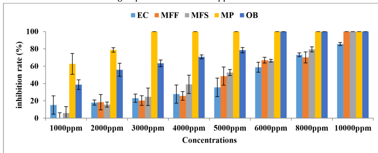
Figure 2: Activity of essential oils on the production of spores of C. gloeosporioides (n = 120, P = 2e-16).
