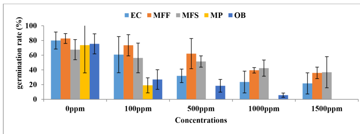
Figure 3: Activity of essential oils on the germination of spores of Colletotrichum gloeosporioides (n = 75, P = 2e-16) EC = Eucalyptus camaldulensis , MFF = Melaleuca quinquenervia (fresh leaves), MFS = Melaleuca quinquenervia (dry leaves), MP = Mentha piperita , OB = Ocimum basilicum
