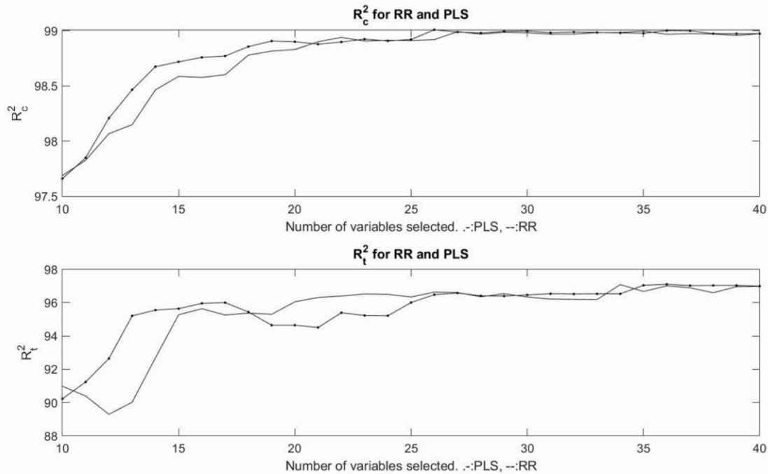
Figure 5. Upper figure R_c^2 -values obtained for RR and PLS at forward selection of variables. Lower figure the R_t^2 -values for test set. .- is those from PLS, -- from RR.
