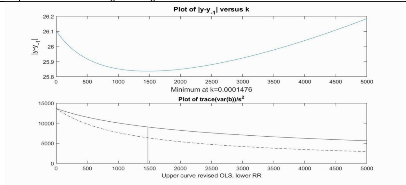
Figure 6. Upper figure a plot of |\hat{\mathbf{y}} - \mathbf{y}_1| versus k. k=i \times 10^{-7} , i=1,2, \dots, 5000 . x-axis is the i-values. Lower figure are plots of (22) and (23). Upper curve for the revised OLS, (22), lower curve for RR, (23).
