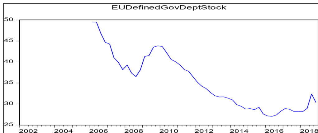
Graph 2. EUDefinedGovDeptStock
